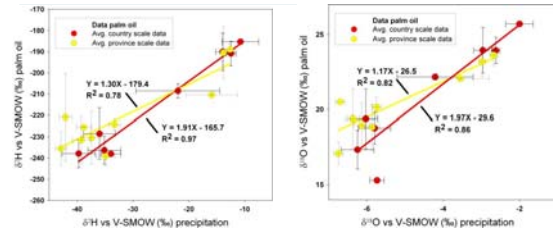
Relation between \delta^2\text{H} in global precipitation and \delta^2\text{H} in palm oil
